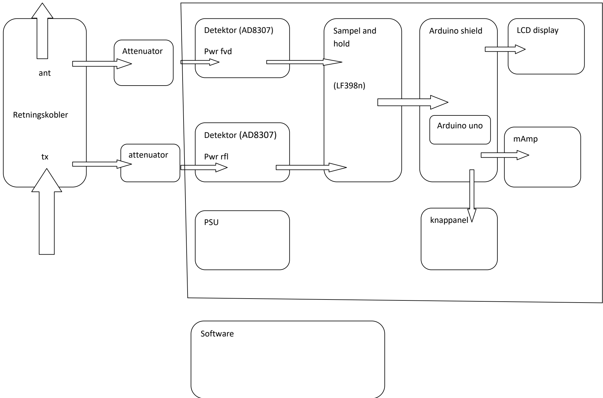
Dual channel powermeter/SWRmeter Blokdigram
